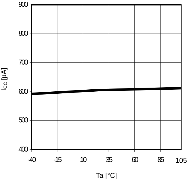
Figure 22. T_a - I_{cc}
