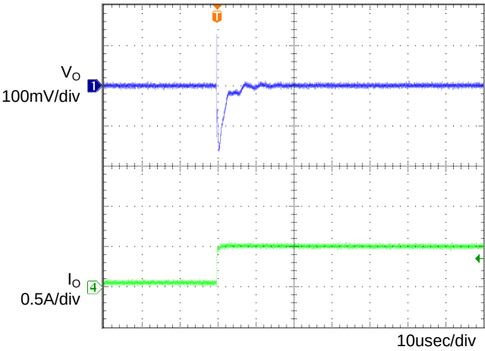
Figure 4. Transient Response (0→0.5A) C_o=1\mu\text{F} , T_a=25^\circ\text{C}
