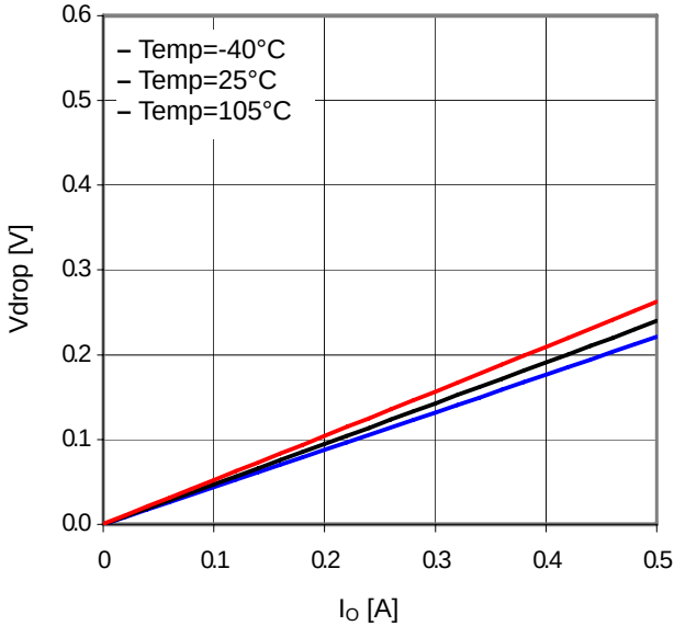
Figure 37. Minimum dropout Voltage 4 ( V_{CC}=10.0V )
