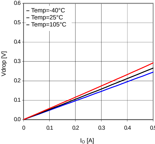
Figure 36. Minimum dropout Voltage 3 ( V_{CC}=8.0V )
