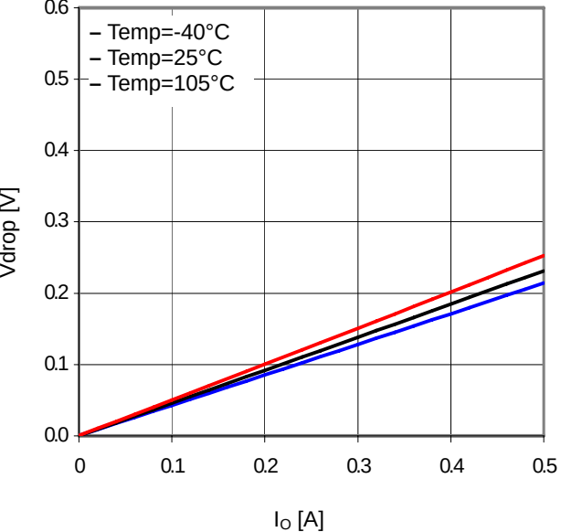
Figure 38. Minimum dropout Voltage 5 ( V_{CC}=12.0V )
