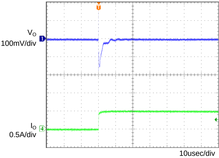
Figure 3. Transient Response (0→0.5A) C_o=1\mu\text{F} , T_a=-40^\circ\text{C}
