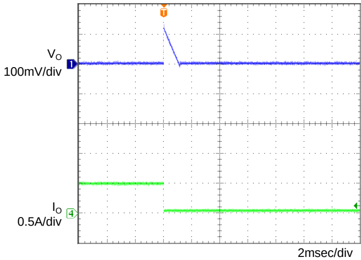
Figure 7. Transient Response (0.5→0A) C_o=1\mu F , T_a=25^\circ C
