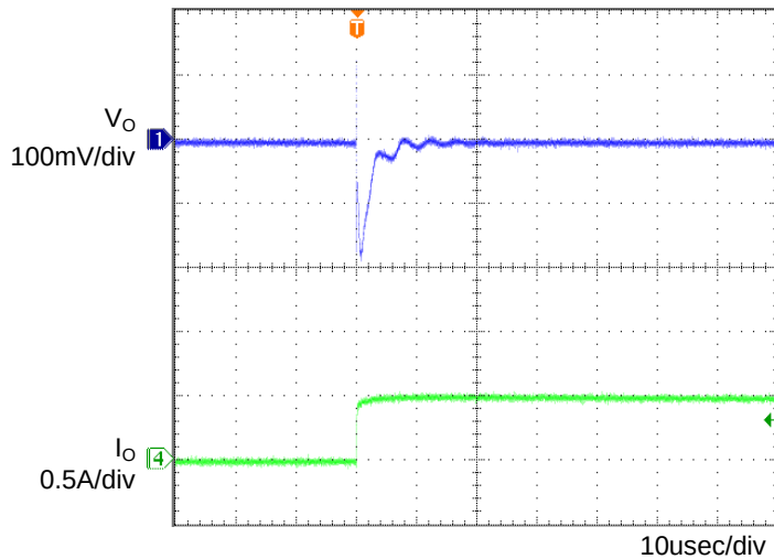
Figure 5. Transient Response (0→0.5A) C_o=1\mu\text{F} , T_a=105^\circ\text{C}
