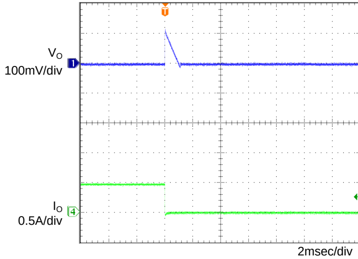
Figure 6. Transient Response (0.5→0A) C_o=1\mu\text{F} , T_a=-40^\circ\text{C}
