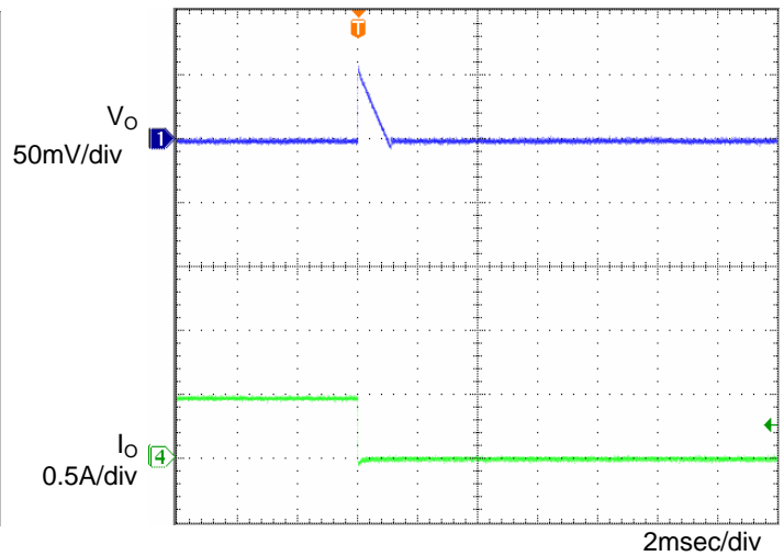
Fig.6 Transient Response (0.5→0A) C_o=1\mu F , T_a=-40^\circ C
