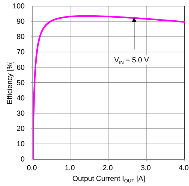
Figure 39. Efficiency vs Output Current (VOUT = 3.3 V)
