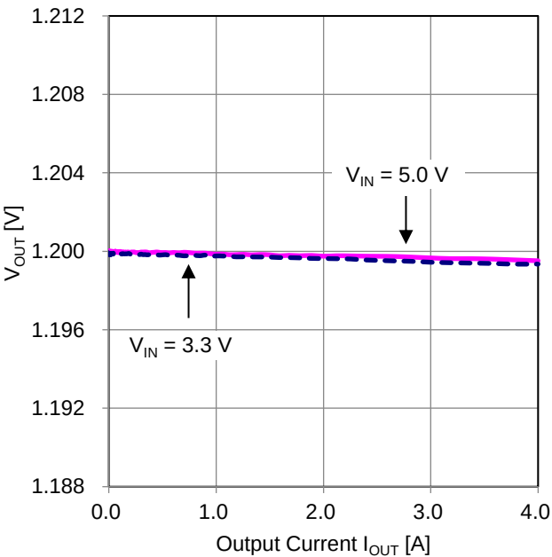
Figure 41. Output Voltage vs Output Current ( V_{OUT} = 1.2 V)
