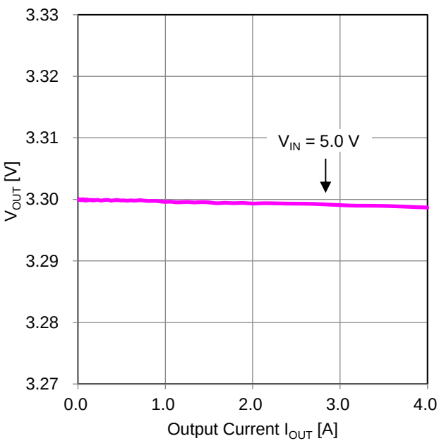
Figure 43. Output Voltage vs Output Current ( V_{OUT} = 3.3 V)
