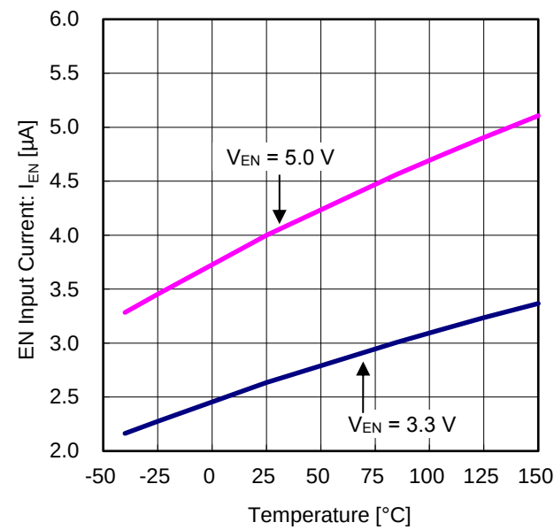
Figure 18. EN Input Current vs Temperature
