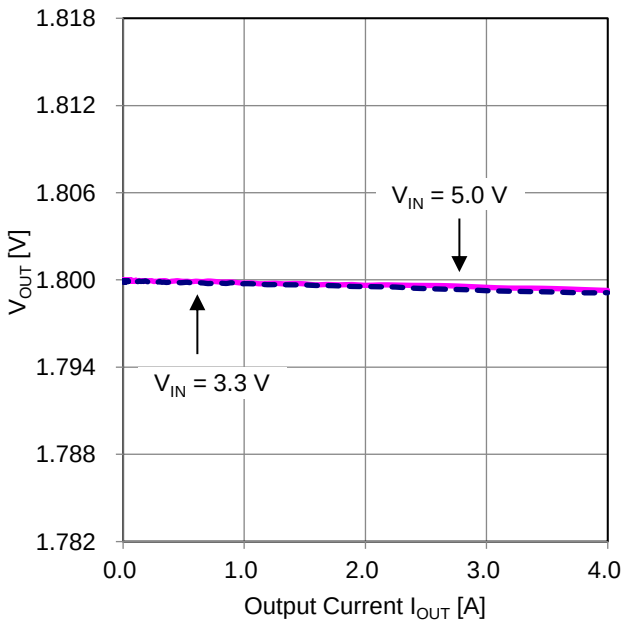
Figure 42. Output Voltage vs Output Current ( V_{OUT} = 1.8 V)
