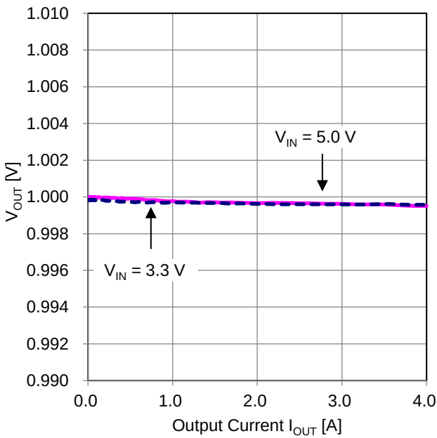
Figure 40. Output Voltage vs Output Current ( V_{OUT} = 1.0 V)
