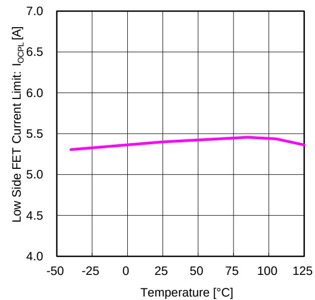
Figure 20. Low Side FET Current Limit vs Temperature
