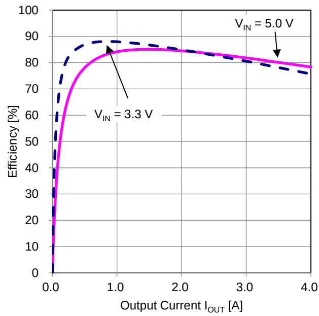
Figure 37. Efficiency vs Output Current (VOUT = 1.2 V)
