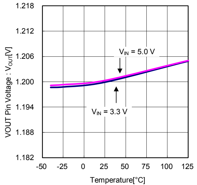
Figure 6. VOUT Pin Voltage vs Temperature (BD9S110NUX-C)
