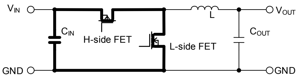
Figure 43-c. Difference of Current and Critical Area in Layout
