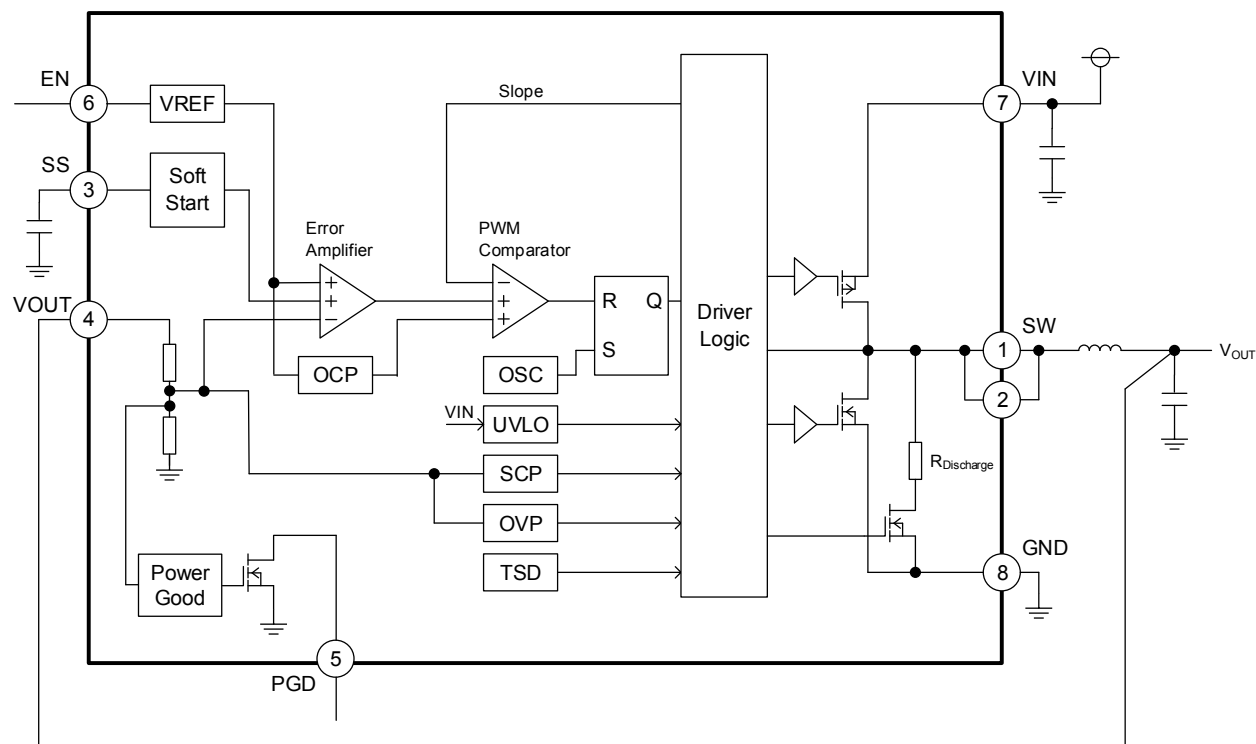
Figure 2. Block Diagram
