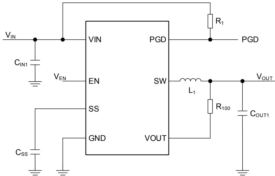
Figure 38. Reference Circuit 2
