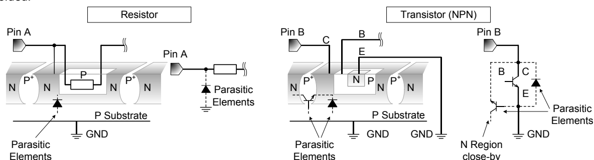
Figure 46. Example of Monolithic IC Structure
