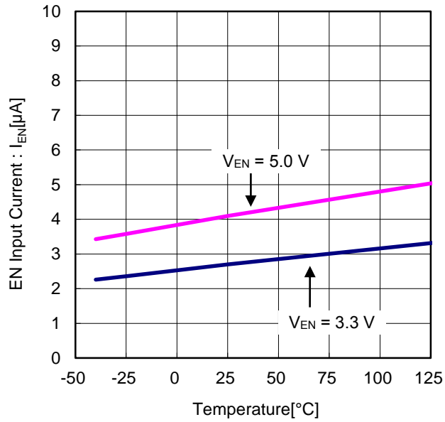
Figure 15. EN Input Current vs Temperature
