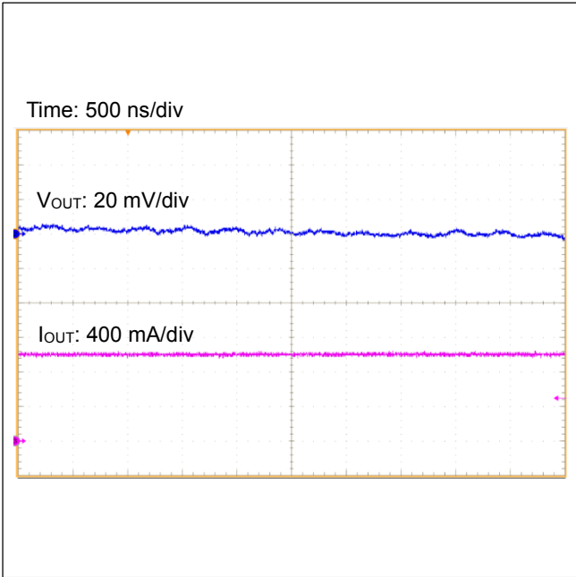
Figure 33. Output Ripple Voltage ( I_{OUT}=1\text{ A} )
