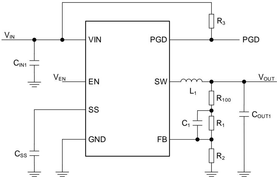
Figure 39. Reference Circuit 3
