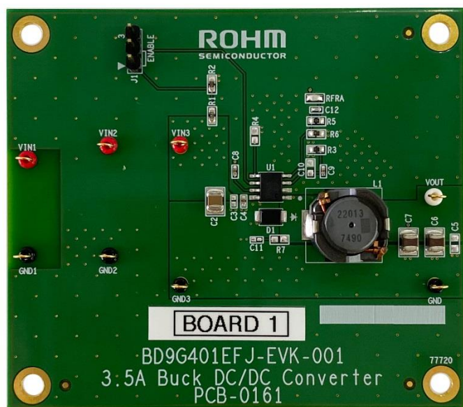
Figure 1. BD9G401EFJ-EVK-001(Top View)
