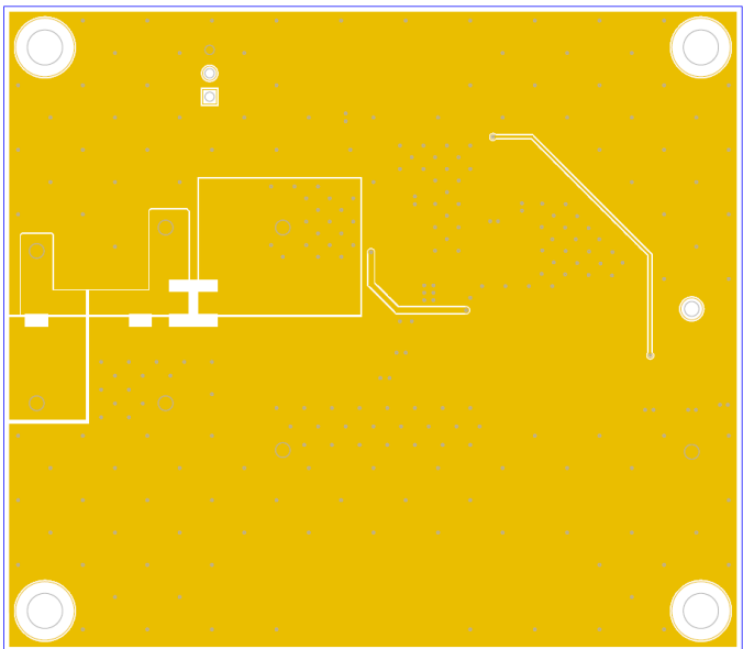
Figure 7. Bottom Layer Layout (Top View)
