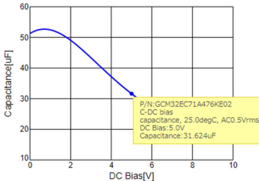
Figure 16. GCM32EC71A476KE02(Murata) DC bias characteristics
