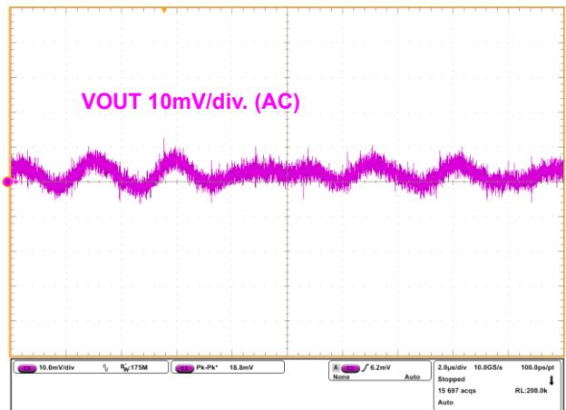
Figure 13. Output Ripple Voltage (VIN=12V, Io=3.5A)
