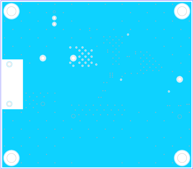
Figure 5. Middle1 Layer Layout (Top View)
