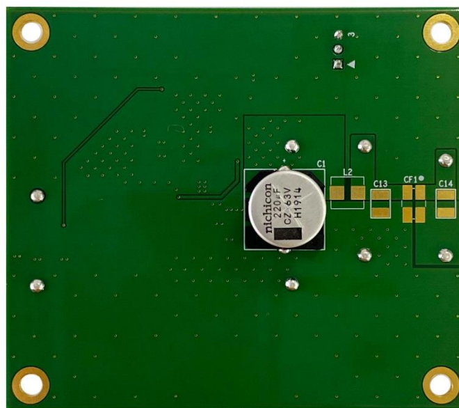
Figure 2. BD9G401EFJ-EVK-001(Bottom View)
