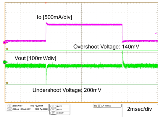
Fig.24 Load Response Iout:100mA \leftrightarrow 1A
