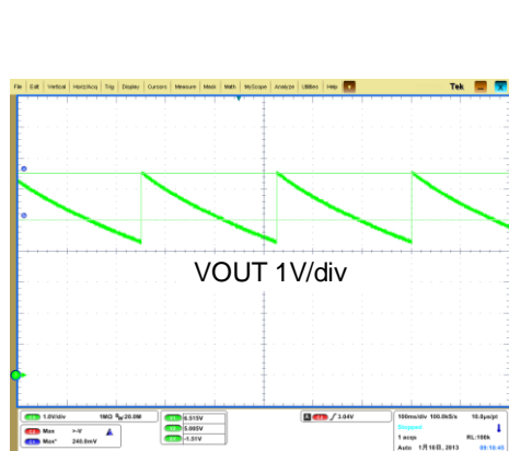
Figure 5. Low voltage and light load, BST-UVLO operation waveform VOUT=5V VCC=7V IOUT=0mA
