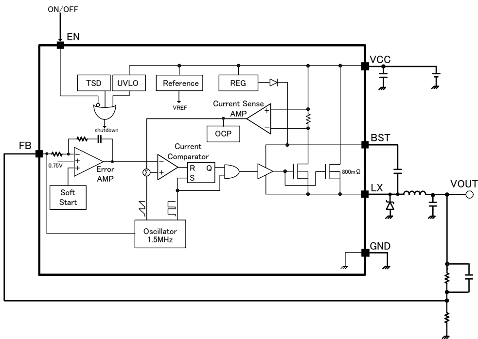
Figure 3. Block Diagram
