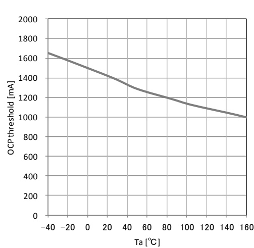
Figure 16. OCP threshold- Temperature
