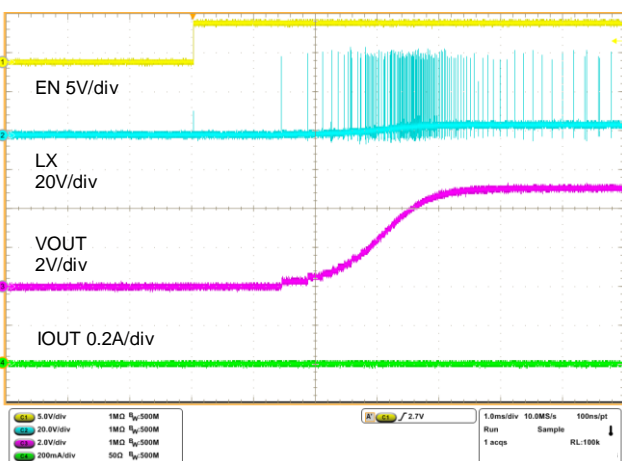
Figure 25. Start-up Characteristics VCC=42V, IOUT=0mA, VOUT=5V
