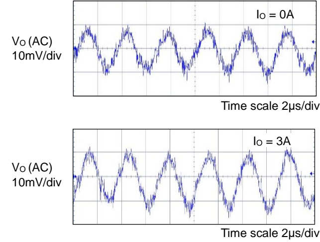
Figure 17. Output Voltage Ripple Wave V_{IN} = 12V , V_O = 5.0V
