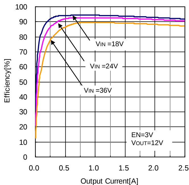
Figure 20. Efficiency vs Output Current ( V_{OUT} = 12V , L = 4.7\mu H )
