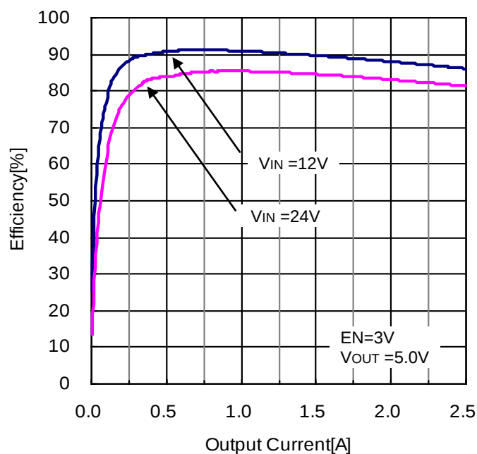
Figure 19. Efficiency vs Output Current ( V_{OUT} = 5.0V , L = 4.7\mu H )
