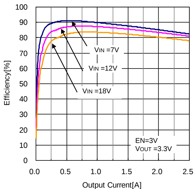
Figure 18. Efficiency vs Output Current ( V_{OUT} = 3.3V , L = 4.7\mu H )
