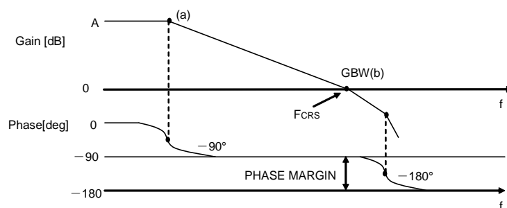
Figure 50. Bode plot
