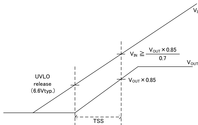
Figure 48. Input Voltage Start-up Time
