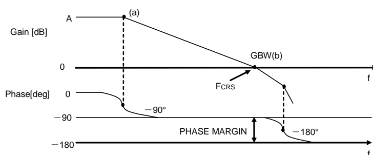
Figure 27. Bode Plot
