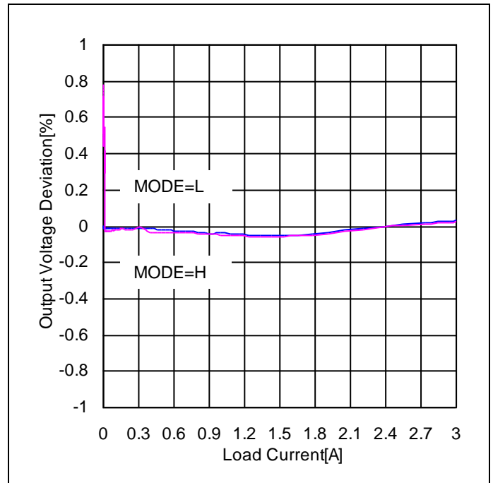
Figure 32. Load Regulation ( V_{IN}=5V , V_{OUT}=1.2V , L=1.0\mu H , FREQ=H )
