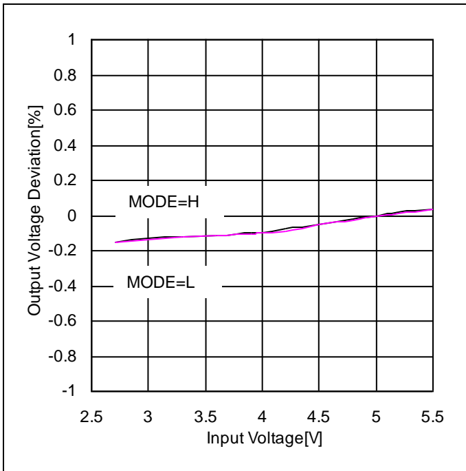
Figure 31. Line Regulation ( V_{OUT}=1.2V , L=1.0\mu H , FREQ=H )
