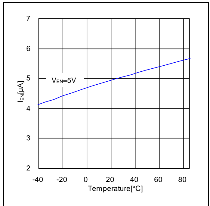
Figure 11. EN Input Current vs Temperature
