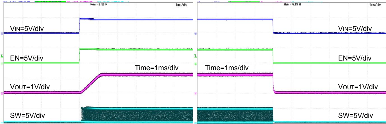
Figure 30. Power Up Waveform with V IN (FREQ=H, RLOAD=0.5Ω)
