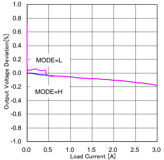
Figure 37. Load Regulation (VIN=5V, VOUT=1.2V, L=1.5 \mu H, FREQ=H)
