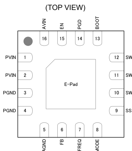
Figure 2. Pin Assignment
