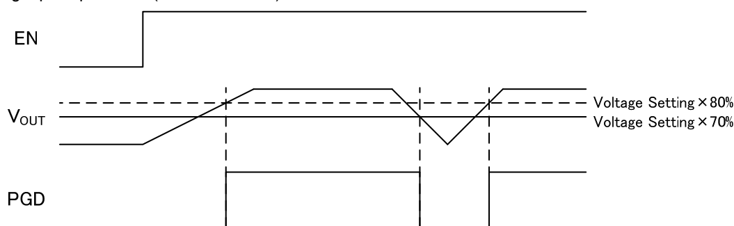
Figure 44. Power Good Timing Chart
