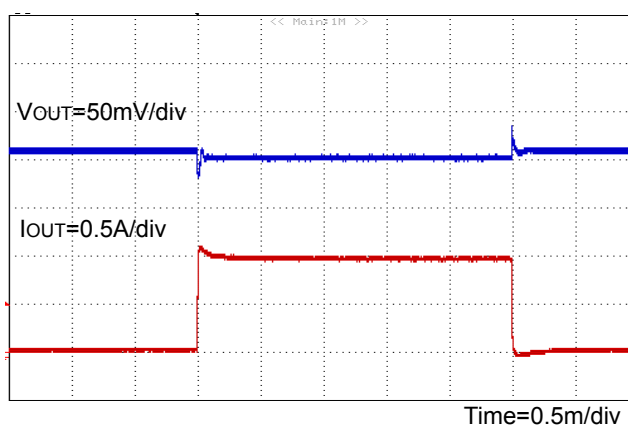
Figure 39. Load Transient Response I_{OUT}=0A to 1A ( V_{IN}=5V , V_{OUT}=1.2V , FREQ=L (2MHz), MODE=H , C_{OUT} =Ceramic 22\mu F )
