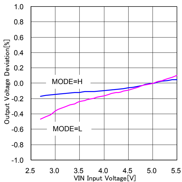
Figure 36. Line Regulation ( V_{OUT}=1.2V , L=2.2\mu H , FREQ=H (1MHz))
