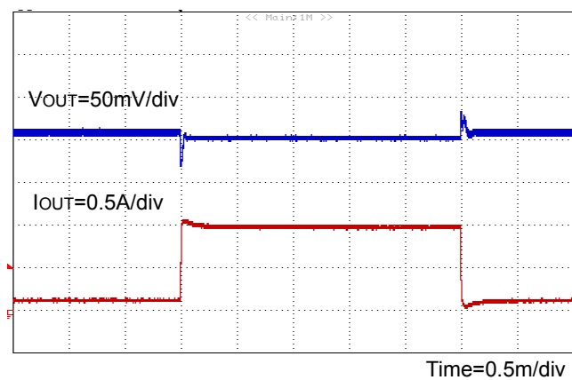
Figure 38. Load Transient Response I_{OUT}=0.1A to 1A ( V_{IN}=5V , V_{OUT}=1.2V , FREQ=L (2MHz), MODE=L , C_{OUT} =Ceramic 22\mu F )
