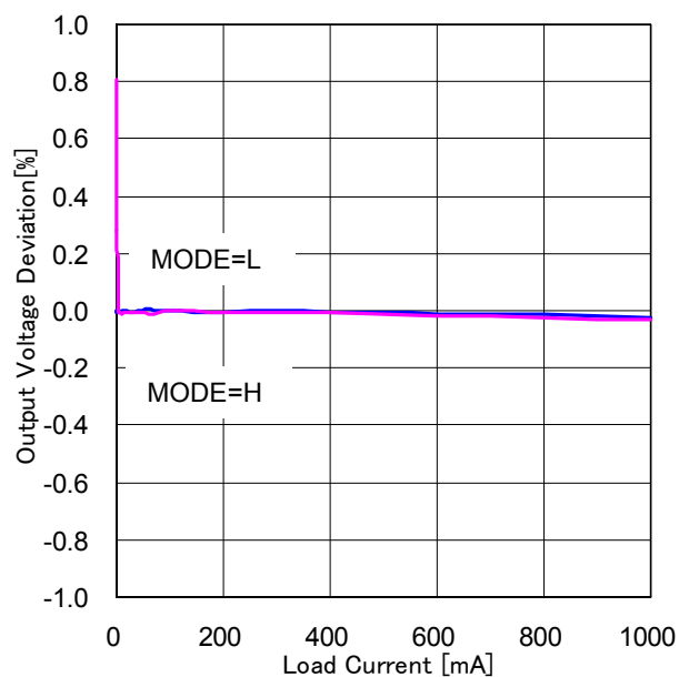
Figure 37. Load Regulation ( V_{IN}=5V , V_{OUT}=1.2V , L=2.2\mu H , FREQ=H (1MHz))
