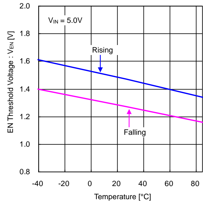
Figure 16. EN Threshold Voltage vs Temperature
