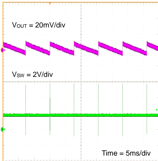
Figure 25. Output Voltage Ripple ( V_{IN} = 5\text{V} , V_{OUT} = 1.8\text{V} , V_{MODE} = V_{IN} , I_{OUT} = 0\text{A} )
