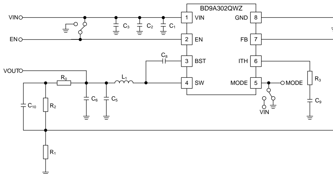
Figure 55. Application Circuit
