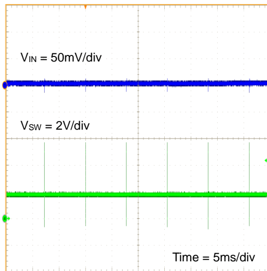
Figure 27. Input Voltage Ripple ( V_{IN} = 5\text{V} , V_{OUT} = 1.8\text{V} , V_{MODE} = V_{IN} , I_{OUT} = 0\text{A} )
