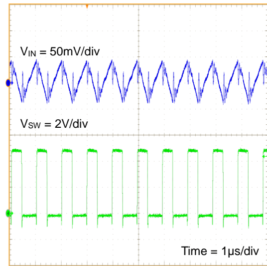
Figure 28. Input Voltage Ripple ( V_{IN} = 5\text{V} , V_{OUT} = 1.8\text{V} , V_{MODE} = V_{IN} , I_{OUT} = 3\text{A} )
