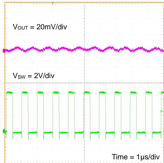
Figure 26. Output Voltage Ripple ( V_{IN} = 5\text{V} , V_{OUT} = 1.8\text{V} , V_{MODE} = V_{IN} , I_{OUT} = 3\text{A} )
