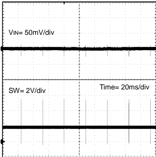
Figure 32. Input Ripple ( V_{IN} = 5\text{V} , V_{OUT} = 1.8\text{V} , I_{OUT} = 0\text{A} )
