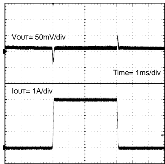
Figure 40. Load Transient Response I_{OUT}=0A to 3A load step ( V_{IN}=5V , V_{OUT}=1.8V , C_{OUT} = Ceramic 44\mu F )
