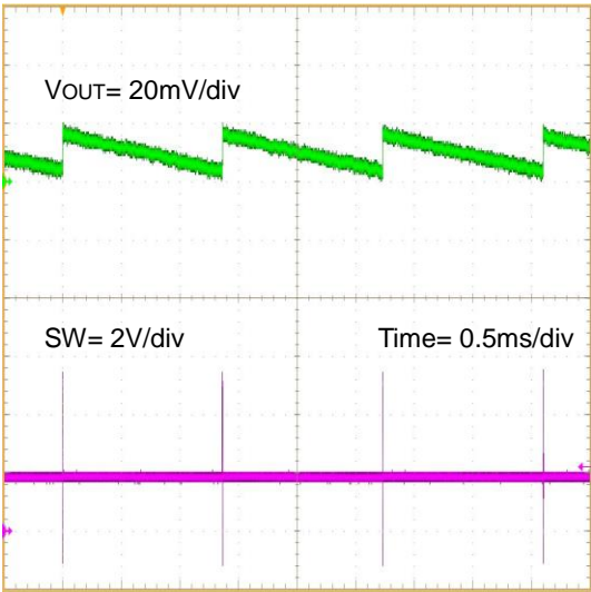
Figure 30. Output Ripple ( V_{IN} = 5\text{V} , V_{OUT} = 1.8\text{V} , I_{OUT} = 0\text{A} )
