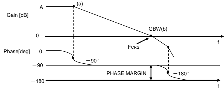
Figure 53. Bode Plot
