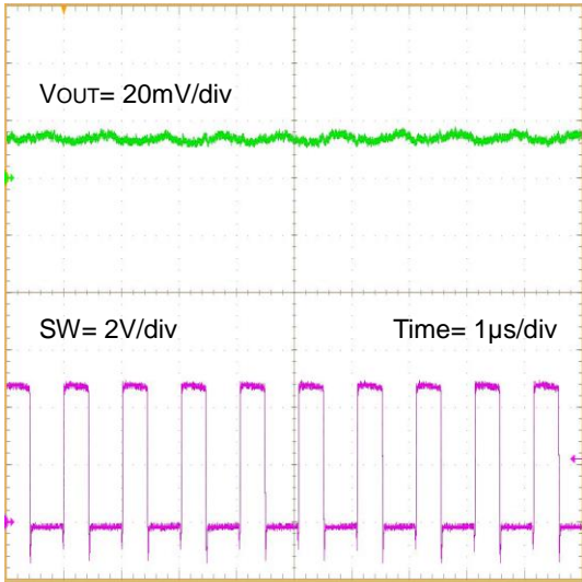
Figure 31. Output Ripple ( V_{IN} = 5\text{V} , V_{OUT} = 1.8\text{V} , I_{OUT} = 3\text{A} )
