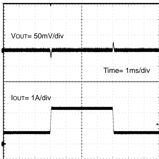
Figure 39. Load Transient Response I_{OUT}=0.75A to 2.25A load step ( V_{IN}=5V , V_{OUT}=1.8V , C_{OUT} = Ceramic 44\mu F )
