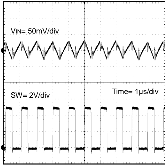
Figure 33. Input Ripple ( V_{IN} = 5\text{V} , V_{OUT} = 1.8\text{V} , I_{OUT} = 3\text{A} )
