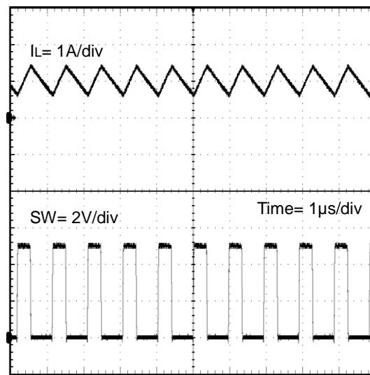
Figure 35. Switching Waveform ( V_{IN}=5.0V , V_{OUT}=1.8V , I_{OUT}=1A , L=1.5\mu H )
