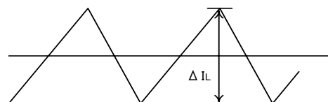
Fig.32 Inductor Current
