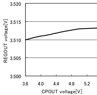
Fig.5 REGOUT Output Line Regulation
