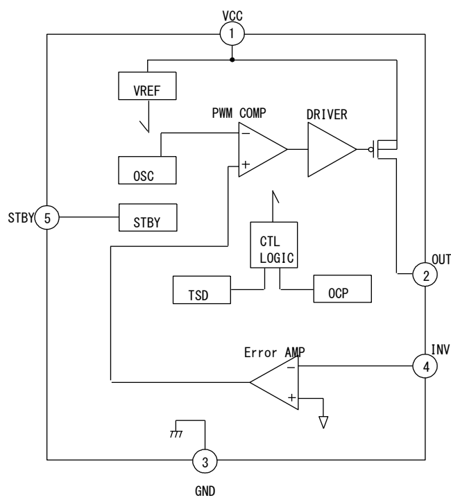
Figure 2. Block Diagram
