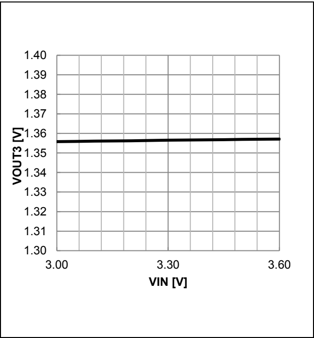
Figure 42. VOUT3 Output Voltage vs VIN (VOUT3 = 1.35 V Setting)
