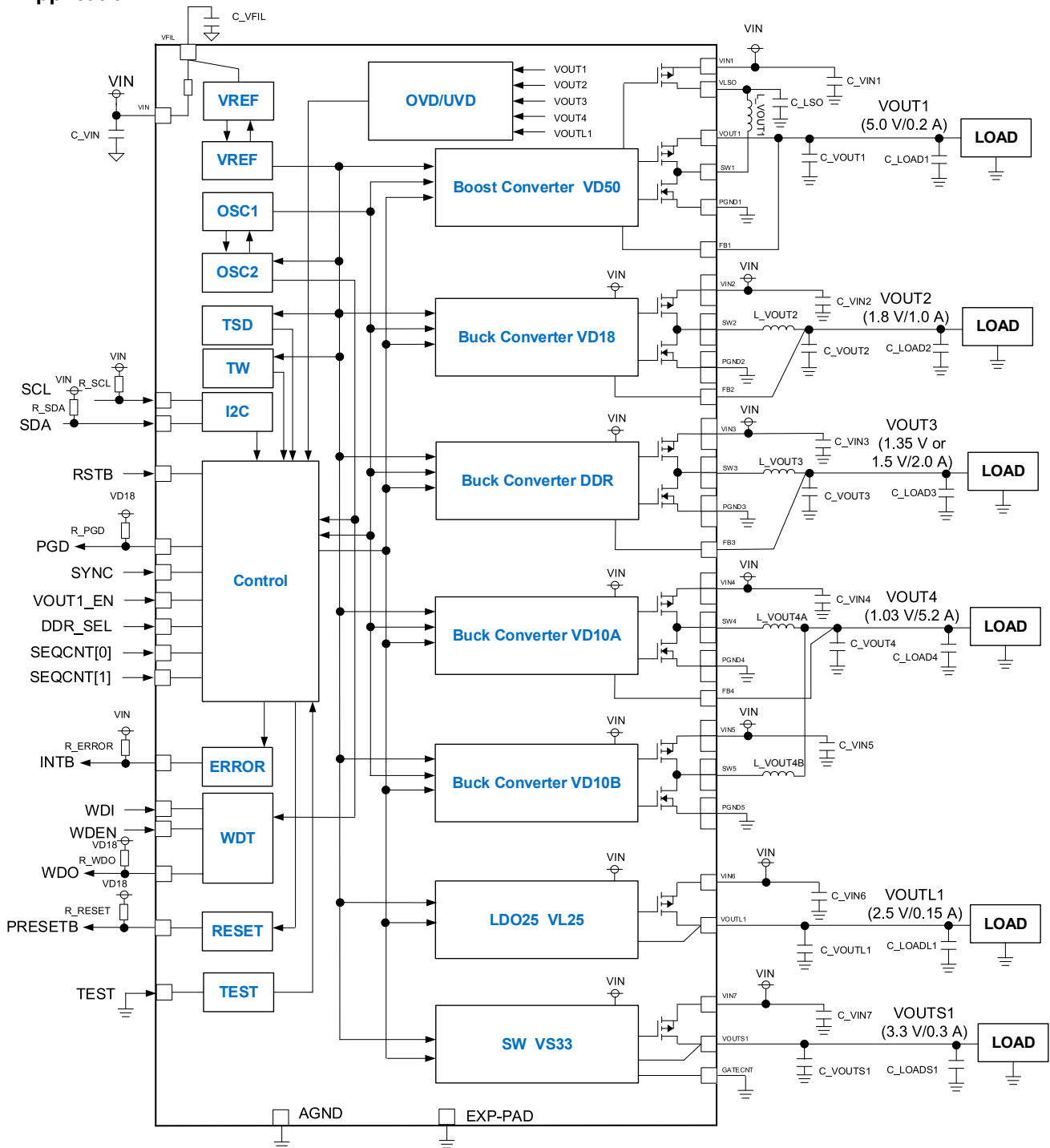
Figure 2. Application Circuit
