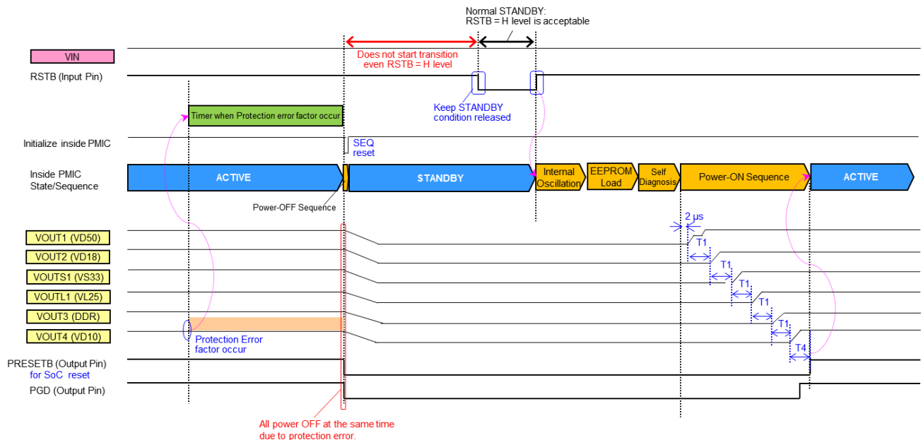
Figure 15. Sequence at Protection Error Occurrence (Timing Chart)
