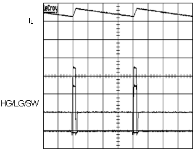
Figure 29. OCP Status ( I_o=5A )
