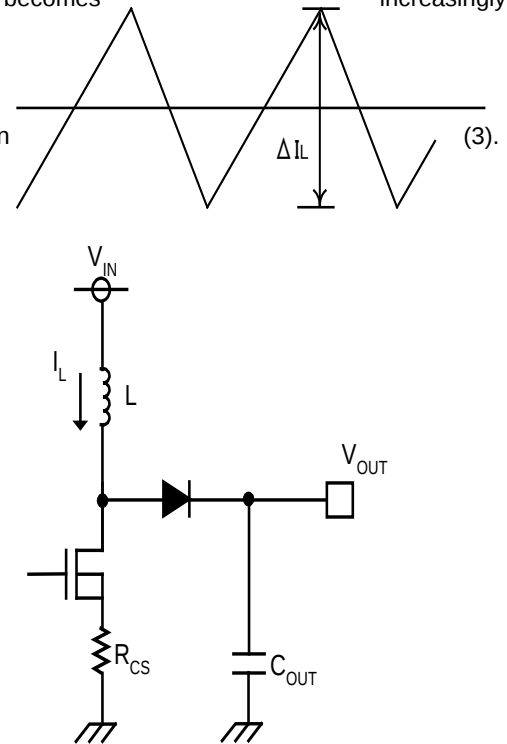
Figure33. DCDC application circuit and coil current
