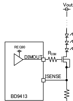
Figure 11. DIMOUT terminal circuit example
