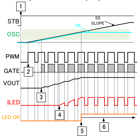
Figure 17. Startup waveform
