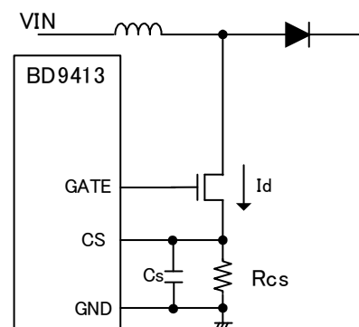
Figure 12. CS terminal circuit example
