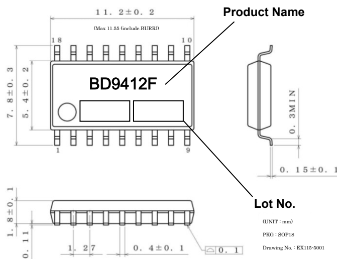
Figure. 4 Physical Dimension and Marking Diagram
