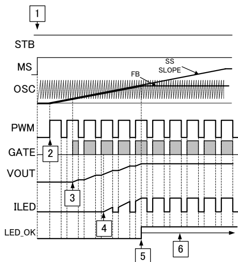
Figure 18. Startup waveform
