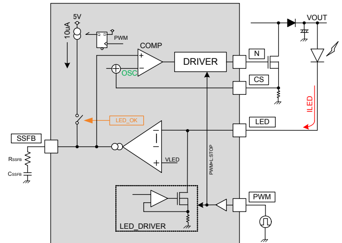
Figure 12. Circuit behavior at startup
