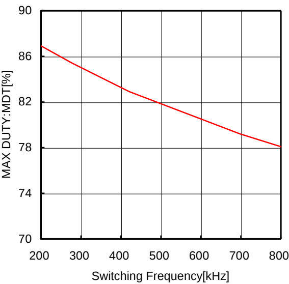
Figure 14. MAX DUTY vs Switching Frequency
