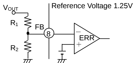
Figure 21. Feedback Resistance Setting
