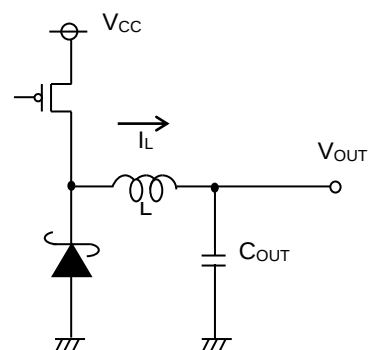
Figure 18. Output Application Circuit (Step Down DC/DC)
