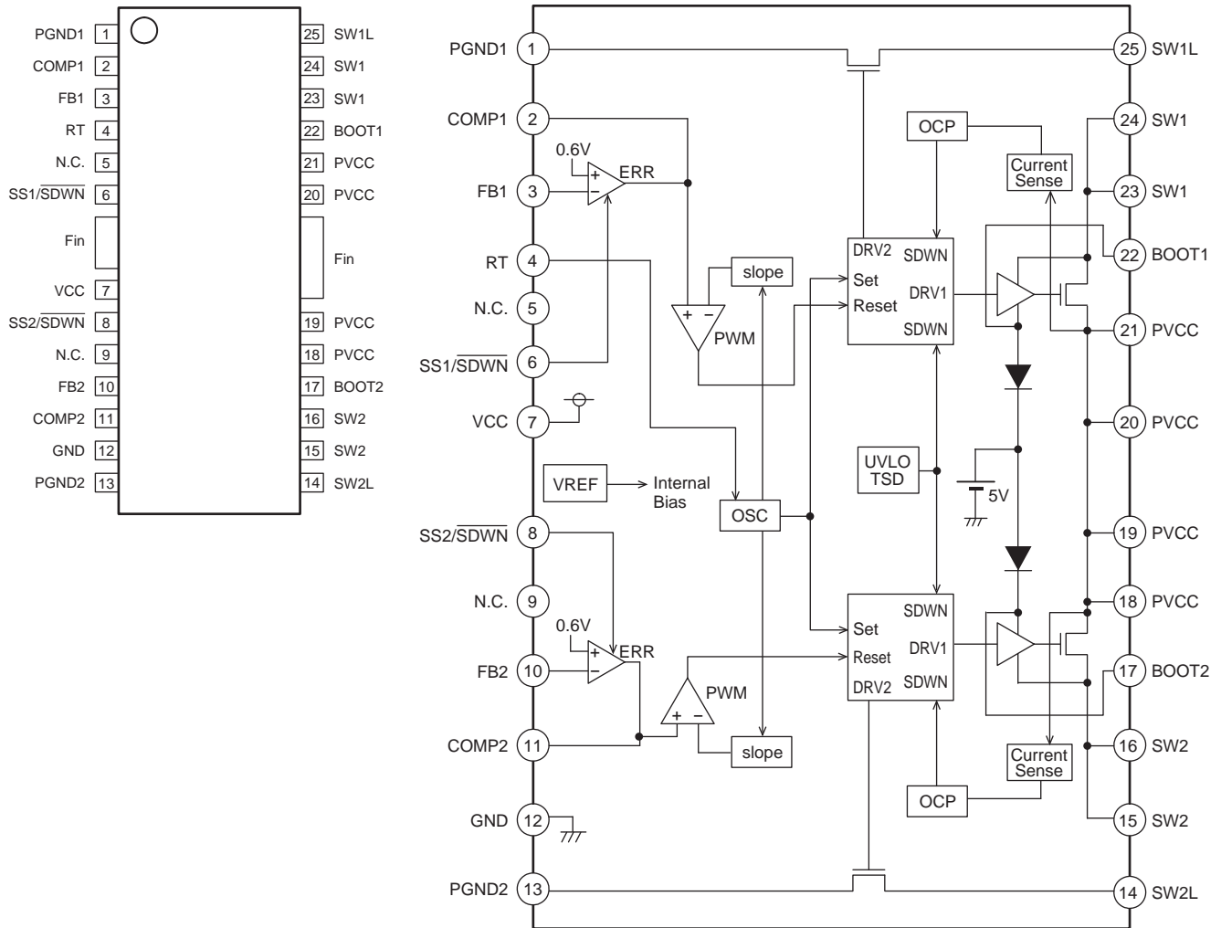
Fig.18 Pin assignment / Block diagram
