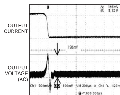
Fig.16 Load transient response No. 2
