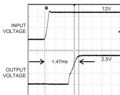
Fig.14 Startup waveform
