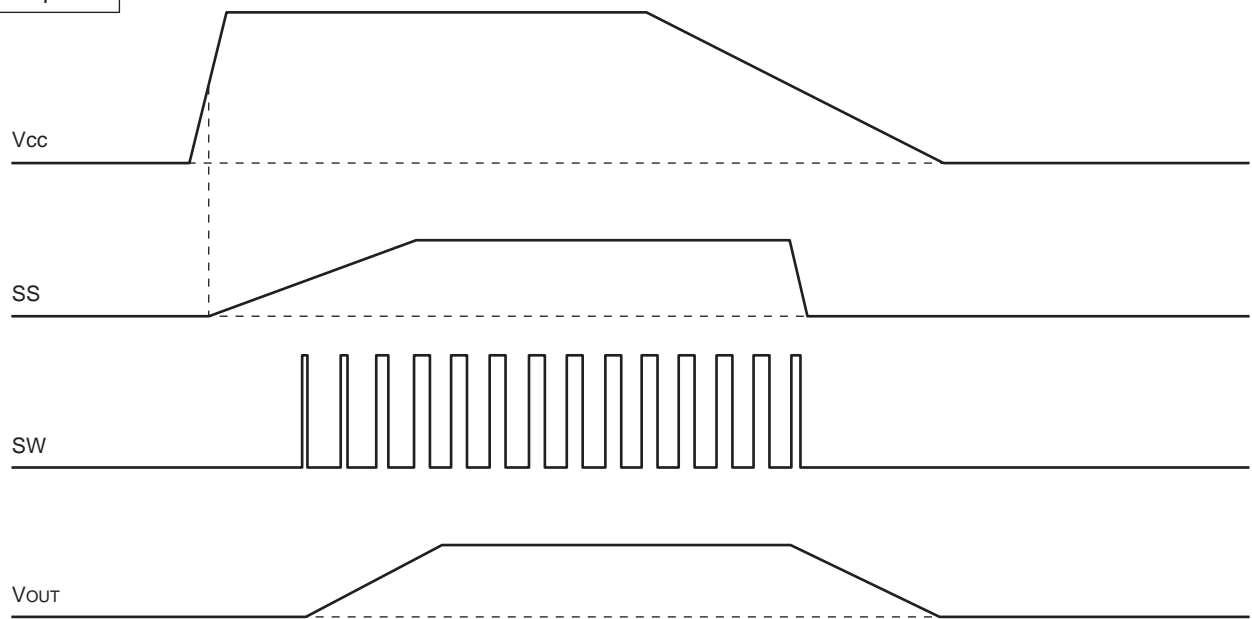
Fig.20 Startup sequence
