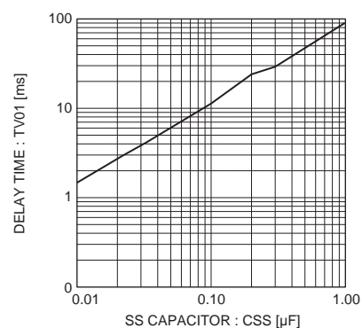
Fig.13 Set capacitance – Delay time
