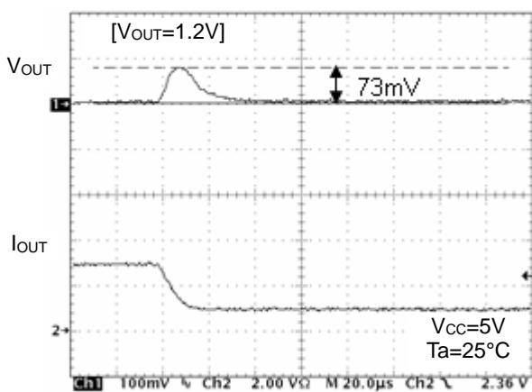
Figure 18. Transient Response ( I_O = 3\text{A} to 1\text{A} , 10\mu\text{s} )
