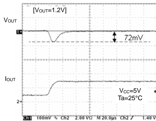
Figure 17. Transient Response ( I_O = 1\text{A} to 3\text{A} , 10\mu\text{s} )
