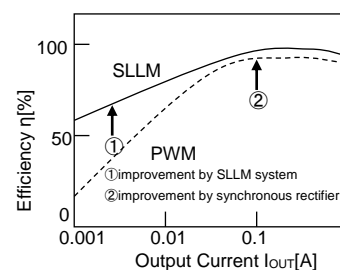
Figure 25. Efficiency
