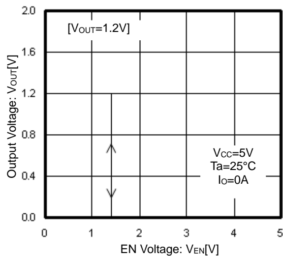
Figure 5. Output Voltage vs EN Voltage
