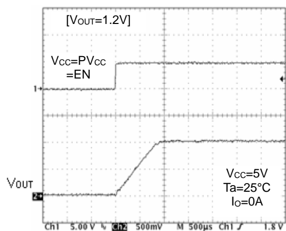
Figure 14. Soft-Start Waveform
