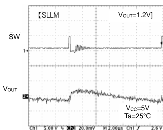
Figure 15. SW Waveform ( I_o=10\text{mA} )
