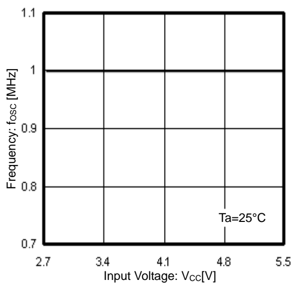
Figure 13. Oscillation Frequency vs Input Voltage
