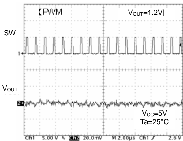
Figure 16. SW Waveform ( I_O = 10\text{mA} )
