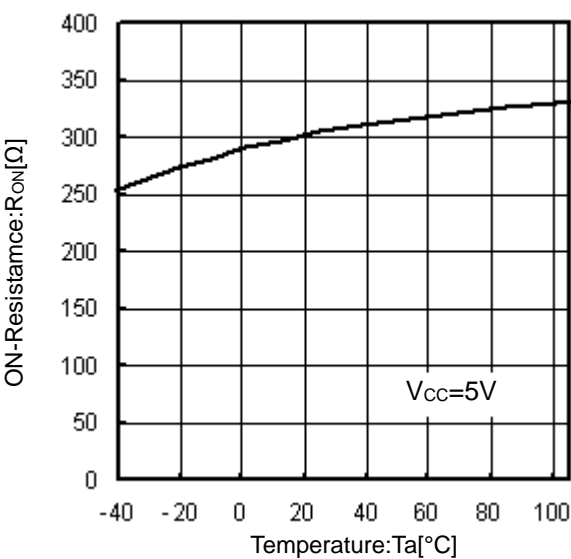
Figure 13. ON-Resistance vs Temperature
