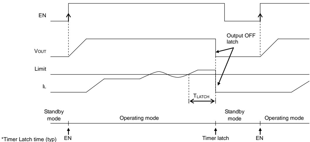
Figure 10 . Short-current protection circuit with time delay timing char
