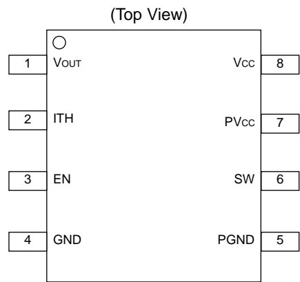
Figure 2. Pin Configuration
