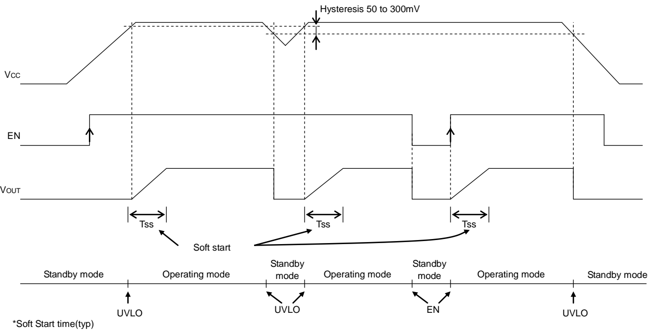
Figure 9 . Soft start, Shutdown, UVLO timing chart
