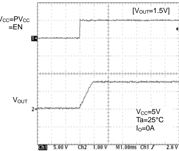
Figure 35. Soft Start Waveform
