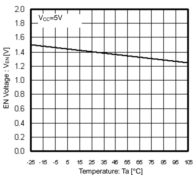
Figure 62. EN Voltage vs Temperature
