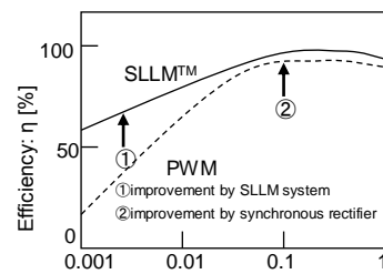
Figure 91. Efficiency
