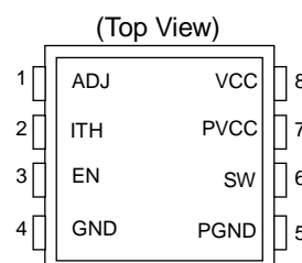
Figure 5. BD9120HFN
