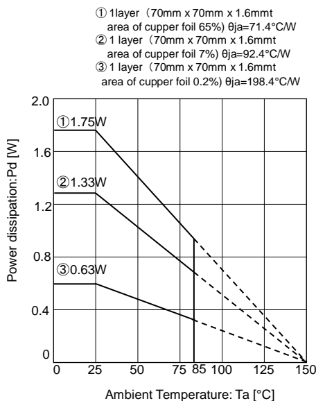
Figure 94. Thermal Derating Curve (HSOP8)
