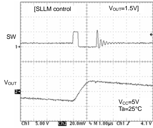
Figure 36. SW Waveform (Io=10mA)
