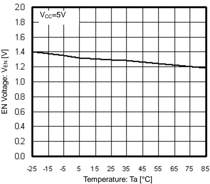
Figure 47. EN Voltage vs Temperature
