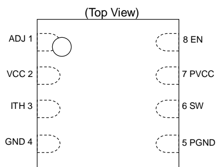
Figure 4. BD9110NV
