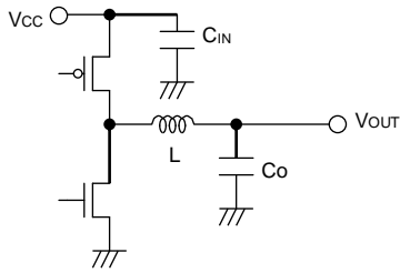
Figure 98. Input Capacitor
