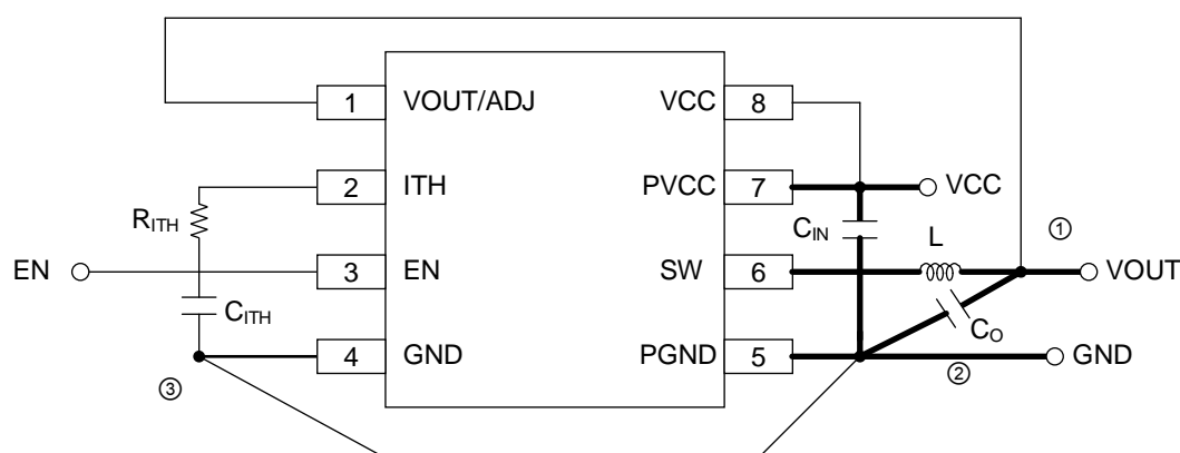
Figure 103. Layout Diagram
