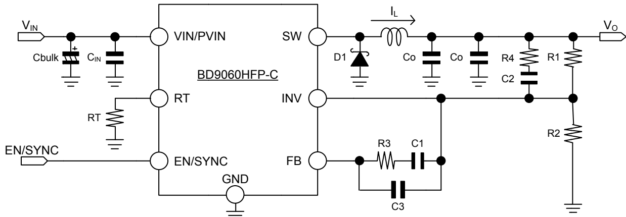
Figure 26. Application Examples 1
