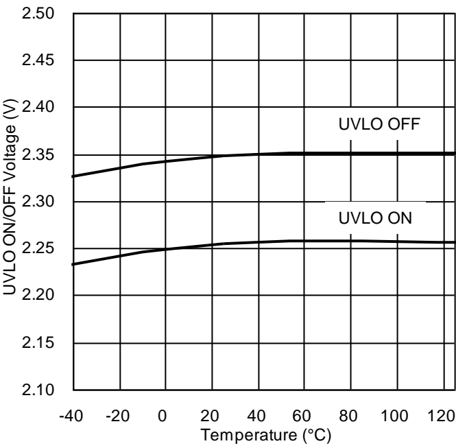
Figure 6. UVLO ON/OFF Voltage vs Temperature
