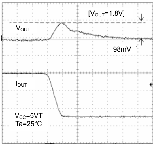
Figure 17. Transient Response ( I_o =600mA to 100mA, 10µs)
