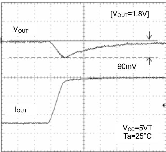
Figure 16. Transient Response ( I_o =100mA to 600mA, 10µs)
