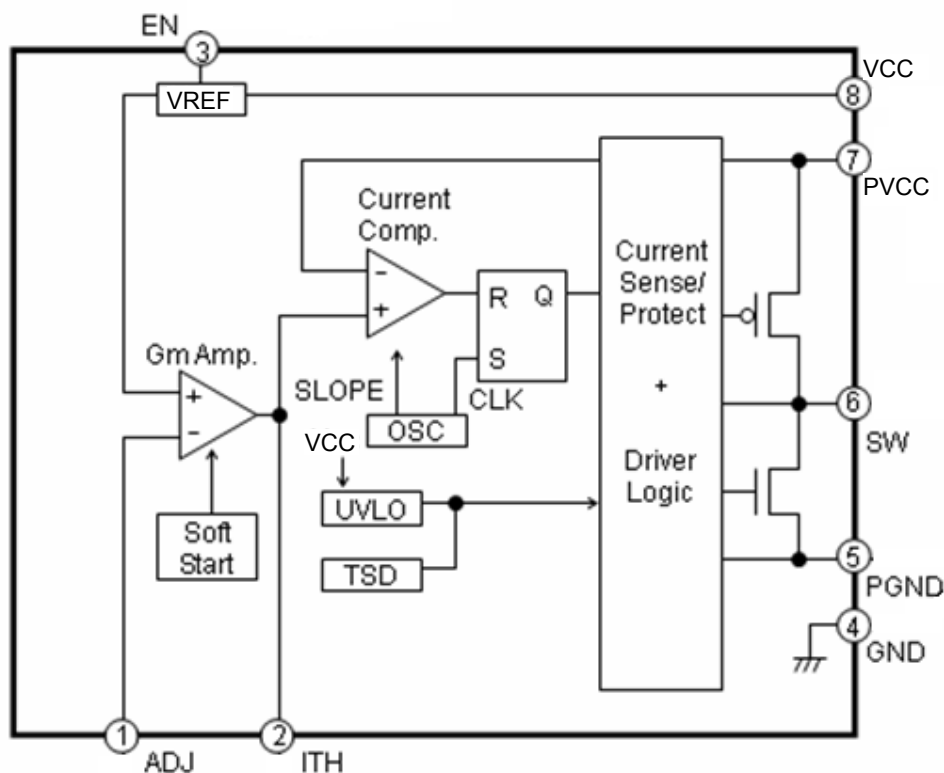
Figure 3. Block Diagram
