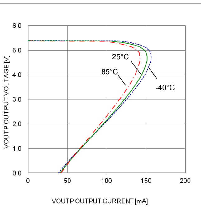
Figure 15. V_{OUTP} vs I_{OUTP} ( T_a -40, 25, 85°C)
