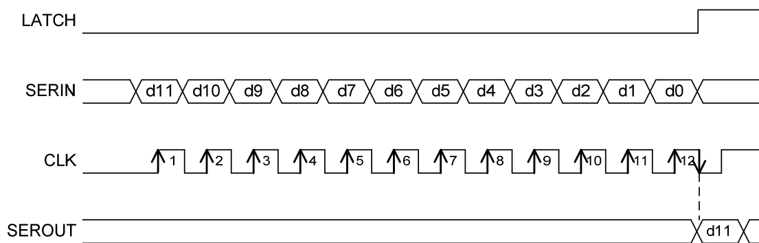
Figure 15. SEROUT Output Signal
