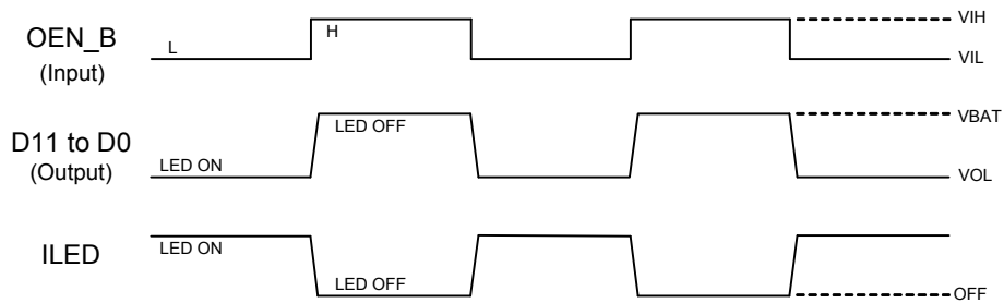
Figure 14. PWM Signal
