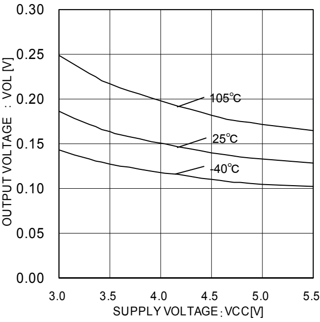
Figure 11. SEROUT low side voltage (VCC characteristic @ ISO=4mA)
