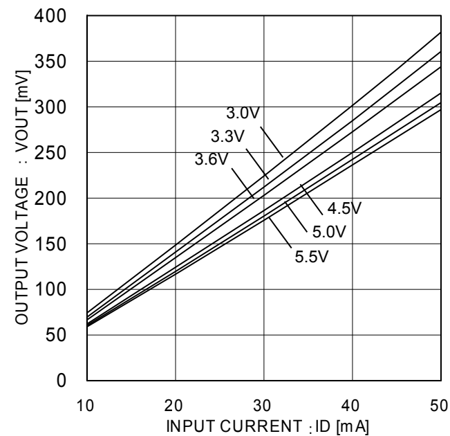
Figure 8. Output ON resistance (ID characteristic)
