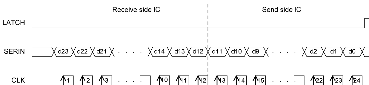
Figure 16. Cascade Connection
