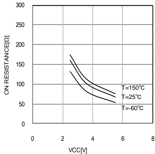
Figure 13. DIS1 discharge SW ON registance vs VCC
