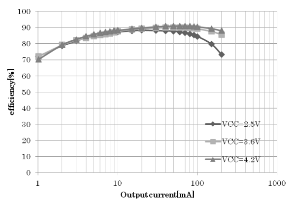
Figure 21. CH2 Power conversion efficiency vs output current
