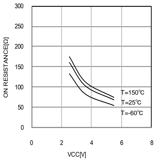
Figure 14. NON1 discharge SW ON registance vs VCC
