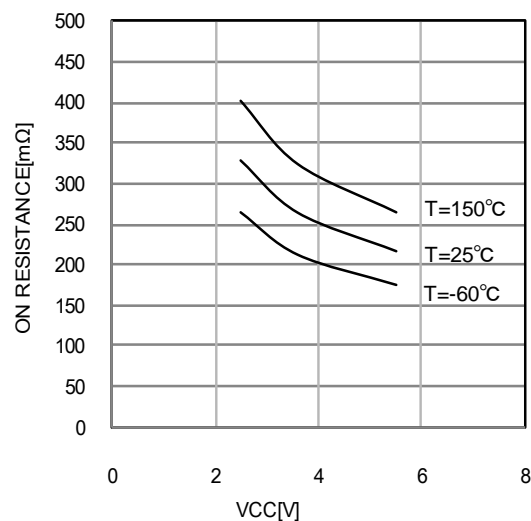
Figure 12. HS2L high side FET ON registance vs VCC
