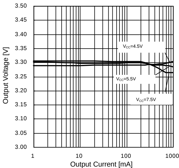
Figure 24. Output Voltage vs Output Current (Load Regulation, V_{OUT} = 3.3V )
