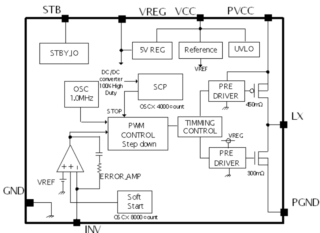
Figure 3. Block Diagram
