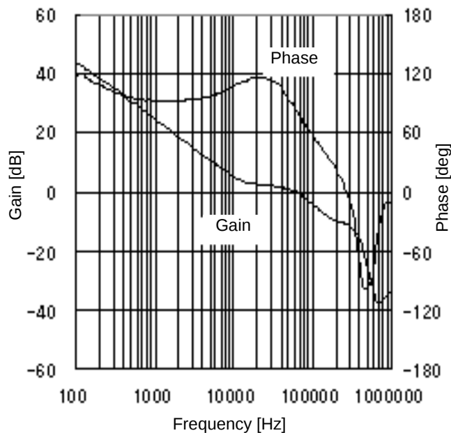
Figure 28. Gain vs Frequency 4 ( V_{CC}=10V , I_O=250mA )
