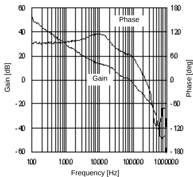
Figure 41. Gain vs Frequency 6 ( V_{CC}=7.4V , I_O=900mA )
