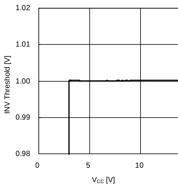
Figure 5. INV Threshold vs V_{CC}
