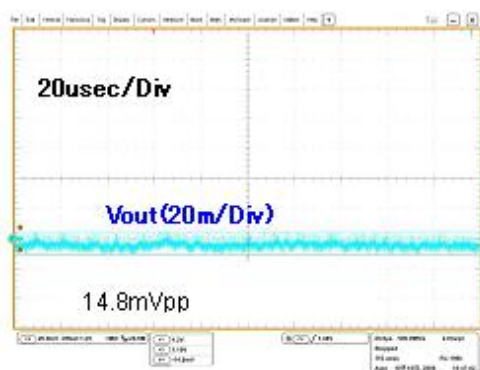
Figure 49. Output Ripple 5 ( V_{CC}=12V , I_o=900mA )
