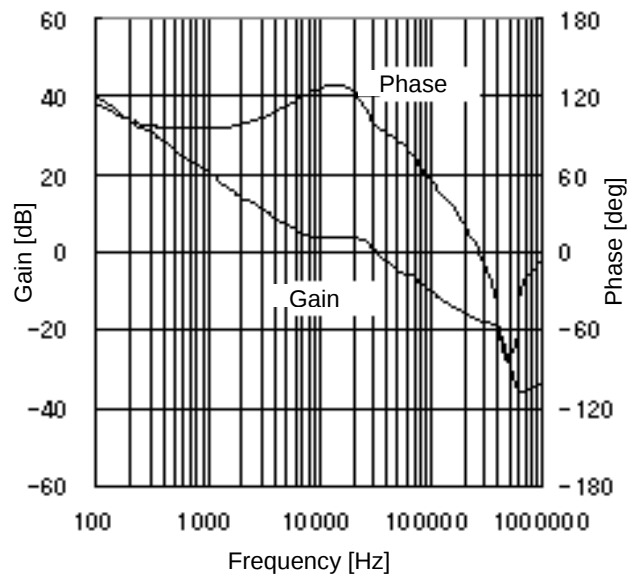
Figure 26 Gain vs Frequency 2 ( V_{CC}=6.0V , I_O=250mA )
