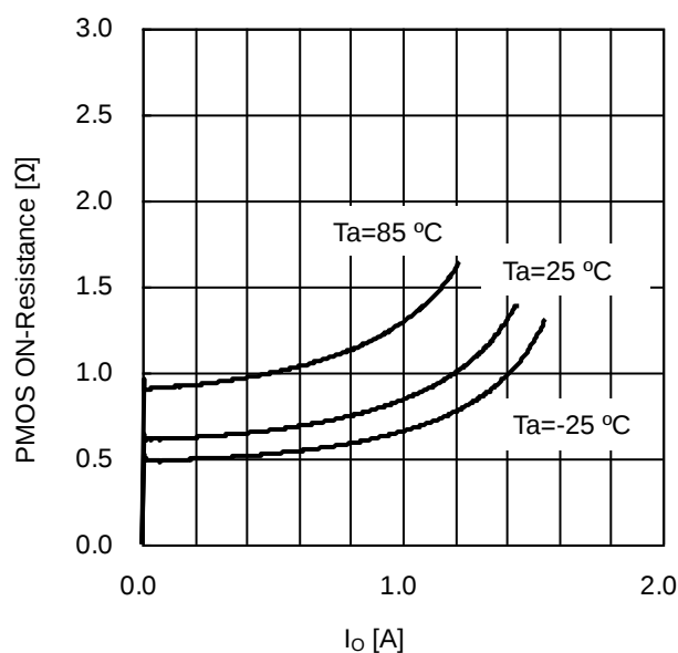
Figure 17. Pch FET ON-Resistance vs I_o ( V_{CC}=4.5\text{V} )
