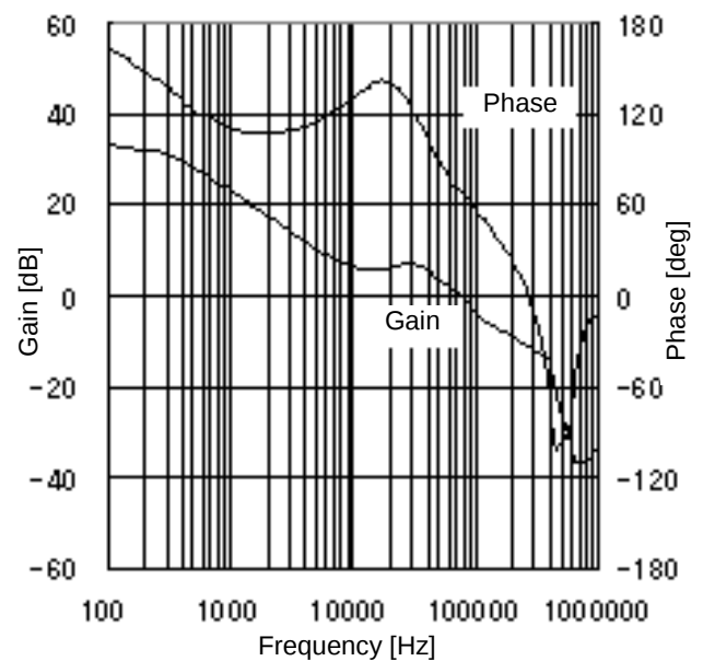
Figure 32. Gain vs Frequency 8 ( V_{CC}=10V , I_o=500mA )
