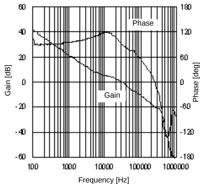
Figure 43. Gain vs Frequency 8 ( V_{CC}=10V , I_O=300mA )
