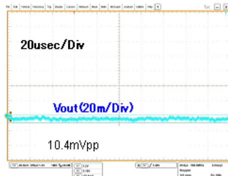
Figure 48. Output Ripple 4 ( V_{CC}=12V , I_o=170mA )
