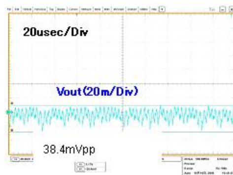
Figure 46. Output Ripple 2 ( V_{CC}=12V , I_o=100mA )
