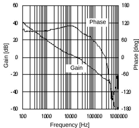
Figure 39. Gain vs Frequency 4 ( V_{CC}=7.4V , I_O=100mA )
