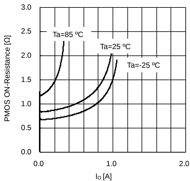
Figure 15. Pch FET ON-Resistance vs I_O ( V_{CC}=3.5\text{V} )
