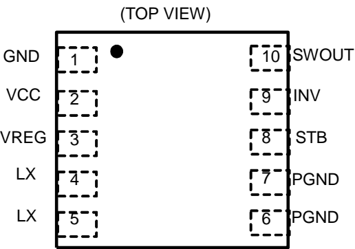
Figure 2. Pin Configuration
