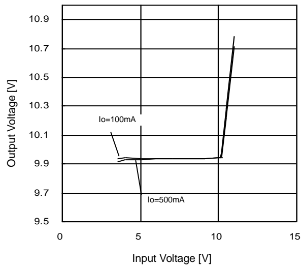
Figure 24. Line Regulation
