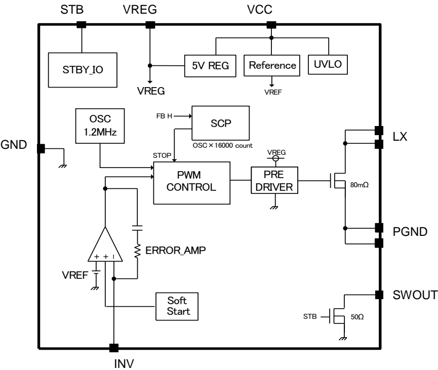
Figure 3. Block Diagram
