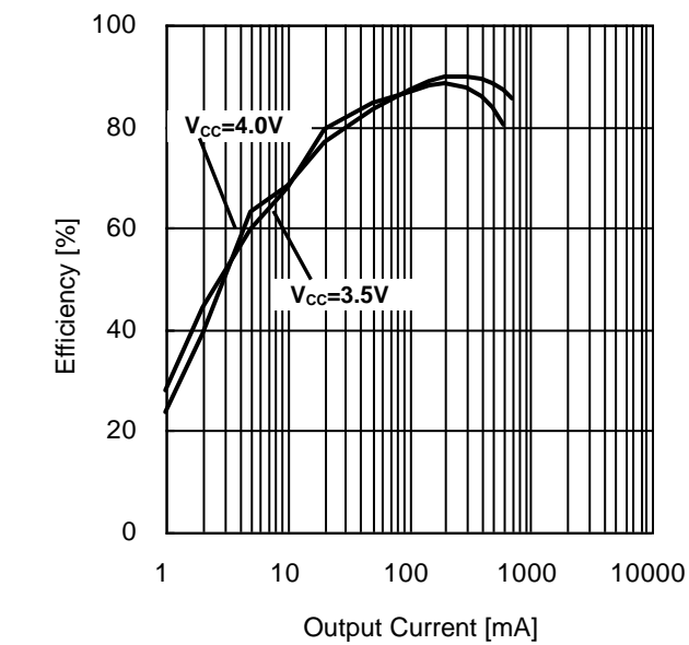
Figure 23. Power Conversion Efficiency3
