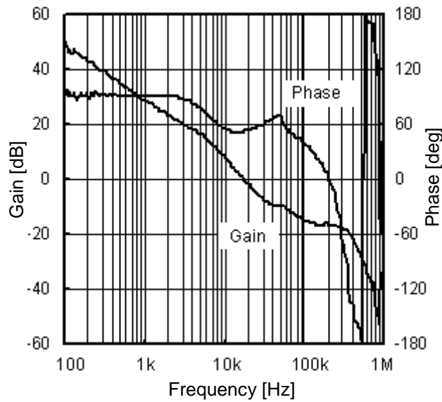
Figure 27. Frequency Response Property 1 ( V_{CC} = 3.5V , I_O = 200mA )
