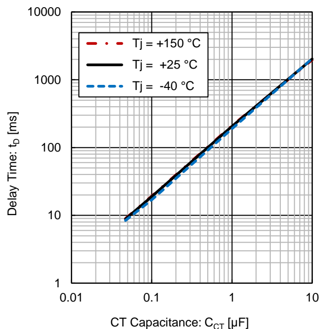
Figure 18. Delay Time vs CT Capacitance
