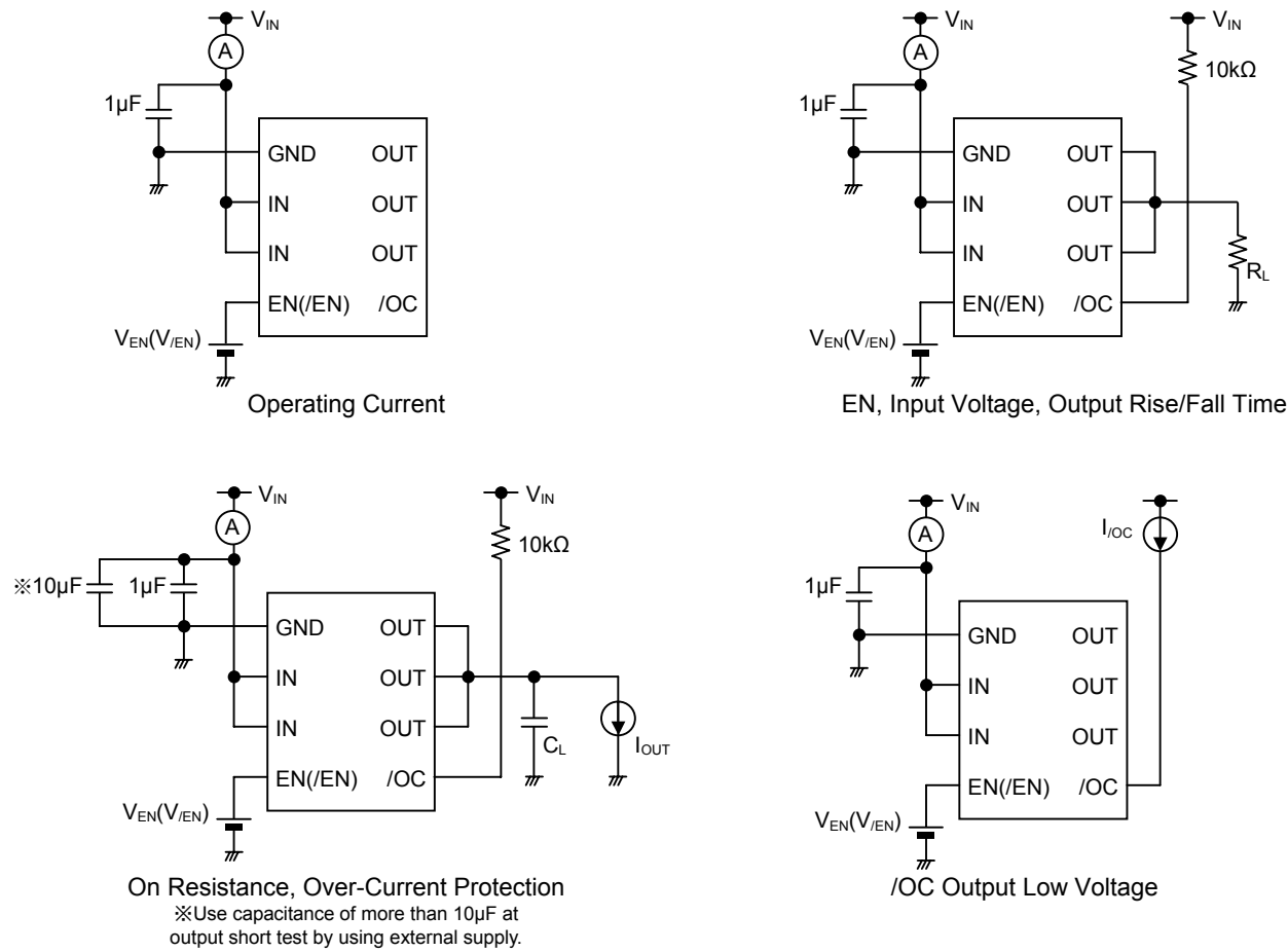
Figure 4. Measurement Circuit
