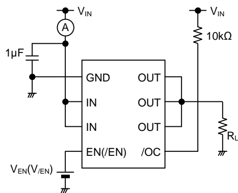
EN, Input Voltage, Output Rise/Fall Time
