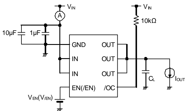
On Resistance, Over-Current Protection
