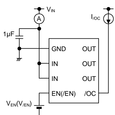
/OC Output Low Voltage
