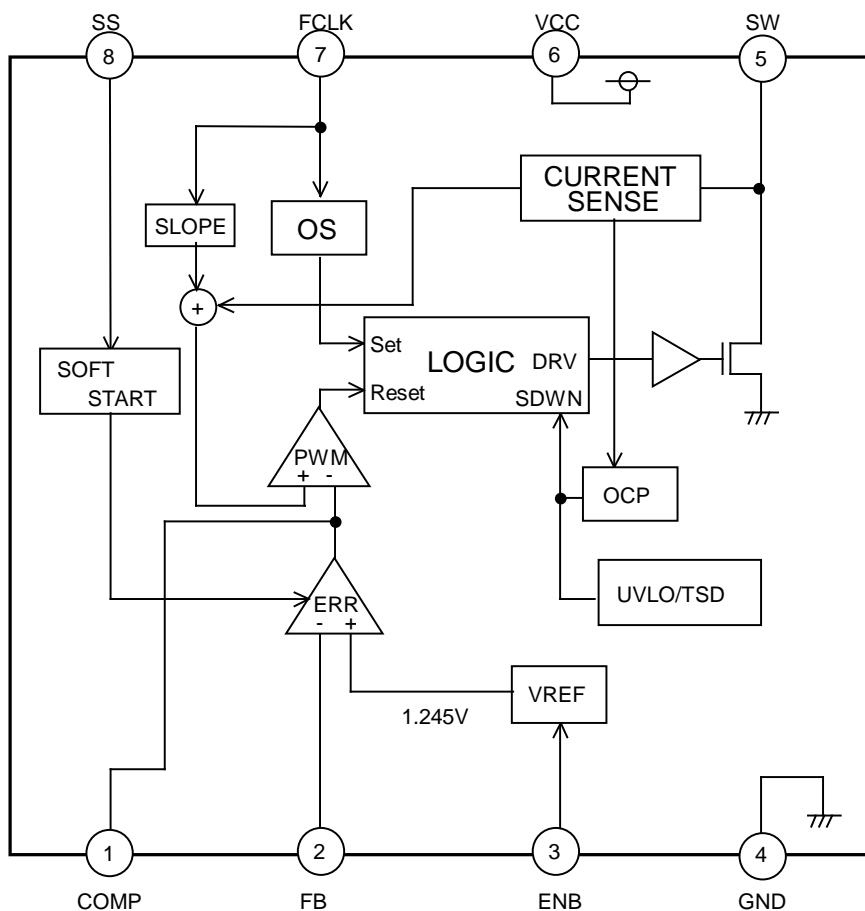
Figure 3. Block Diagram
