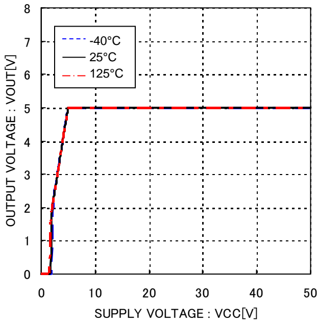
Figure 17. Output voltage vs. Supply voltage IOU=100mA
