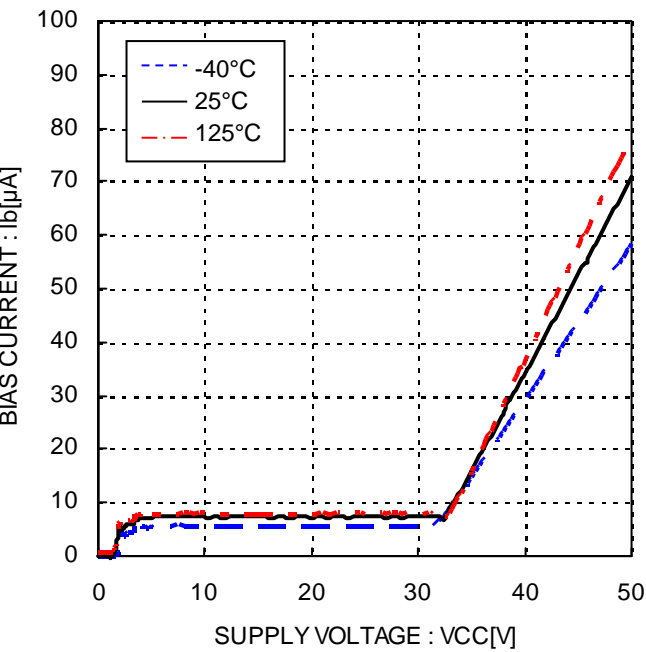
Figure 15. Bias current
