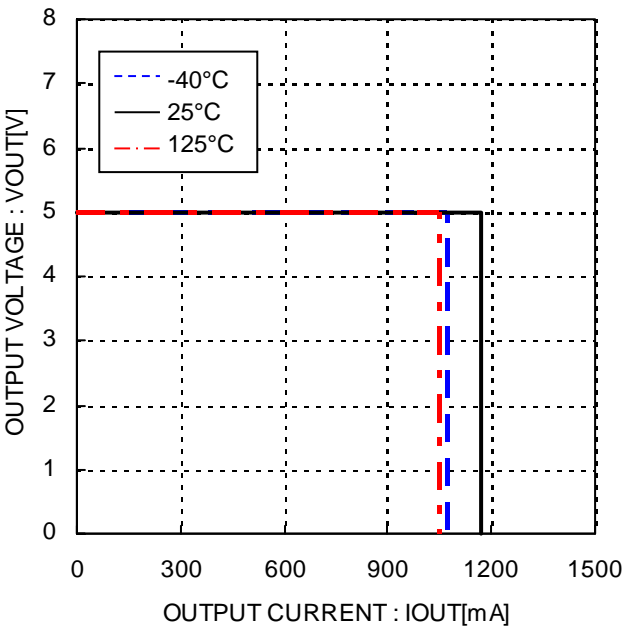
Figure 18. Output voltage vs. Load
