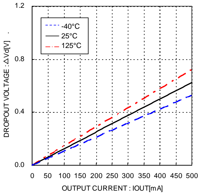
Figure 19. Dropout voltage
