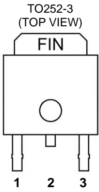
Figure 3. Pin Configuration
