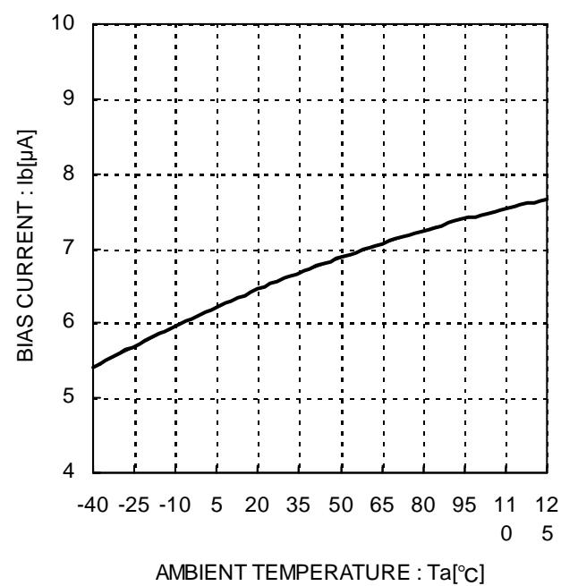
Figure 24. Bias current vs. Temperature
