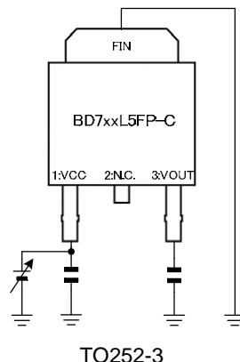
TO252-3 Figure 2. Typical Application Circuits
